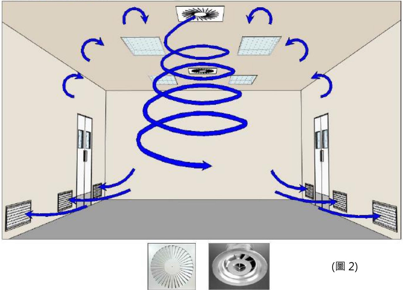
Figure 20. Swirl diffuser
