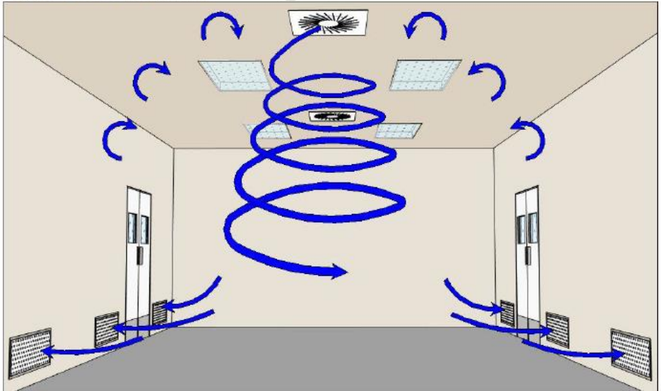
Figure 20. Swirl diffuser
