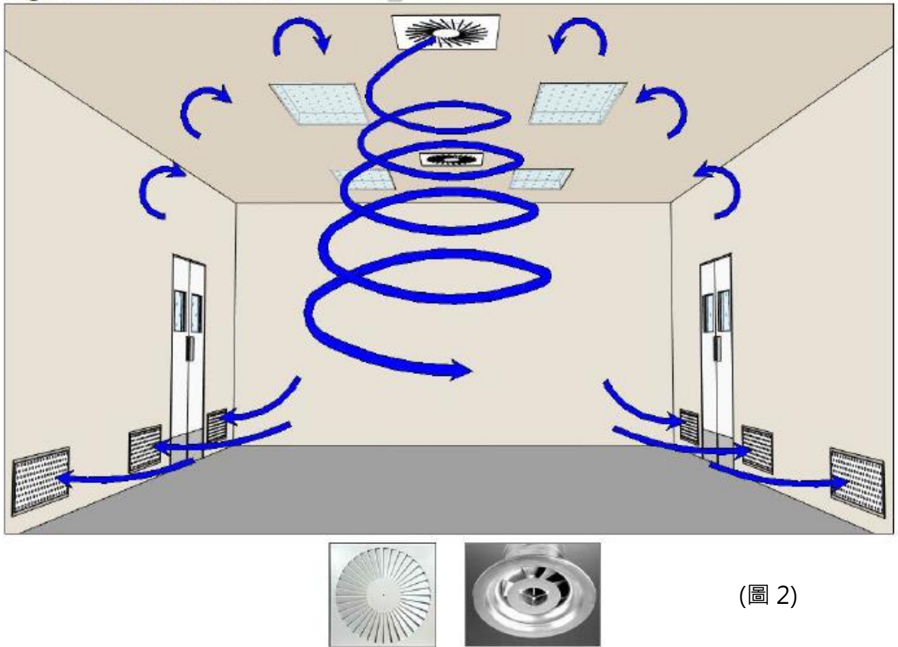
Figure 20. Swirl diffuser
